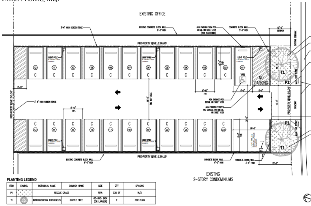
Parking Layout
