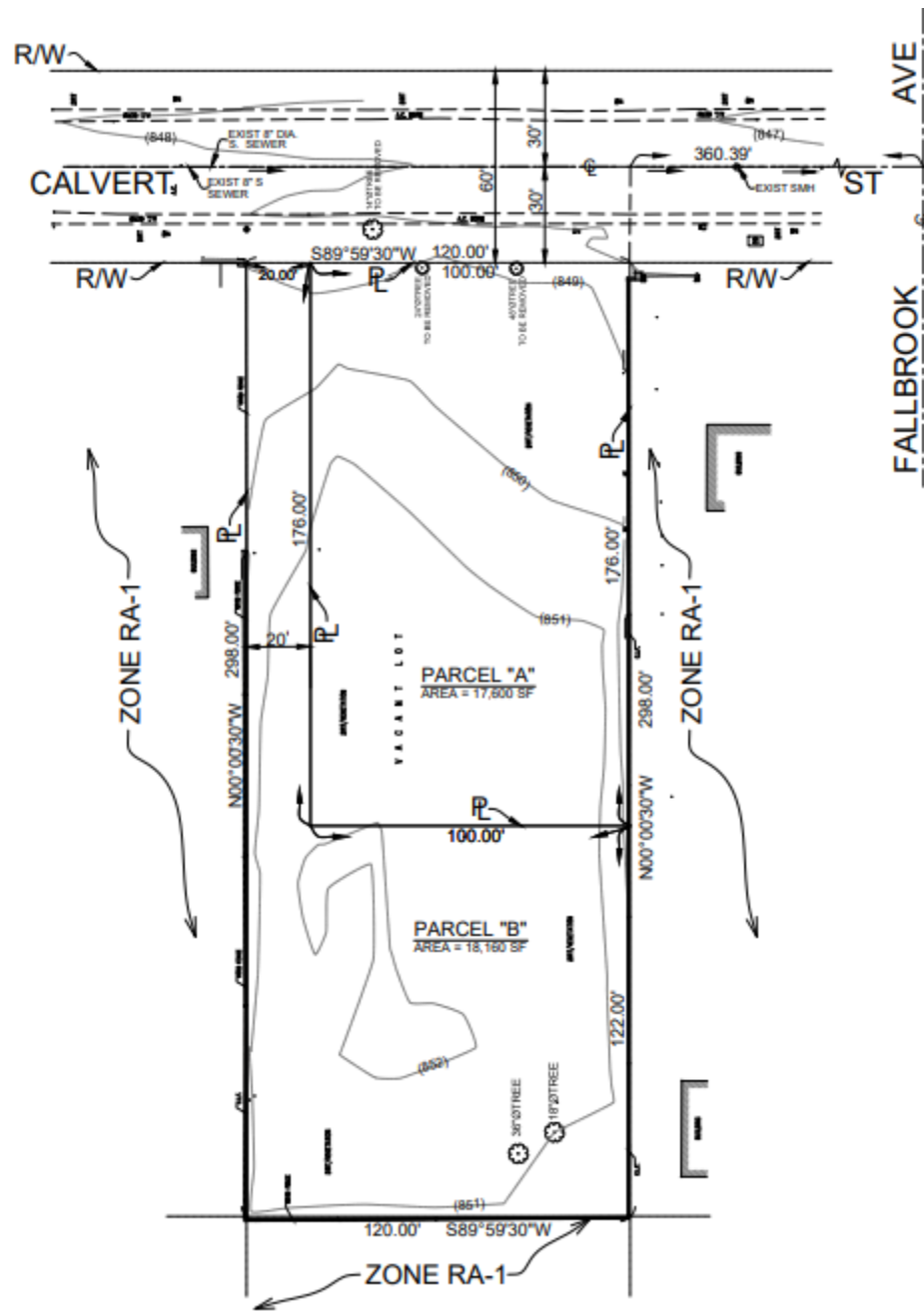
Preliminary Parcel Map for 22840 Calvert Street
